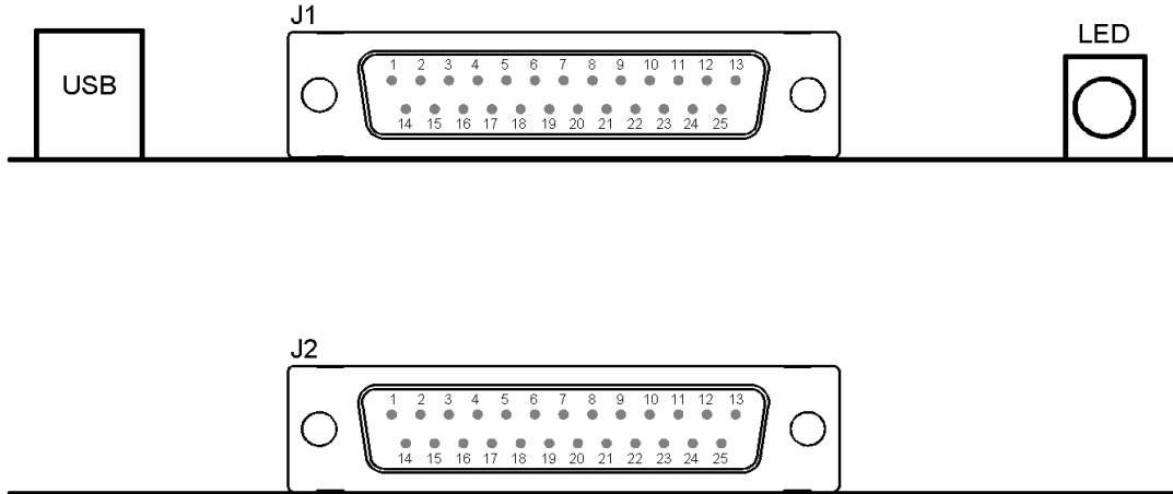
Connector Locations on each end of Module 25 pin Sub "D" male
